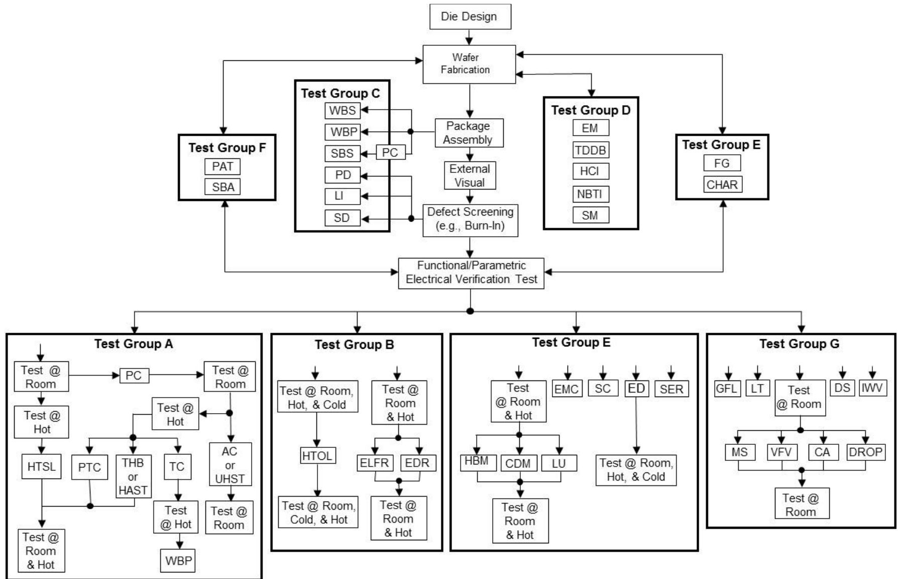
Figure 2: Qualification Test Flow
